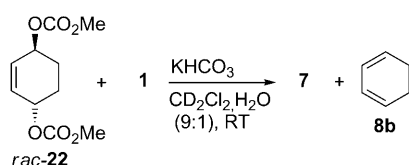
Scheme 12. Redox reaction of complex 1 with biscarbonates 5 and rac - 22 with formation of complex 7 and diene 8 .
