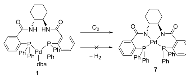
Scheme 11. Oxidation of the Pd 0 complex 1 to the Pd II complex 7 with dioxygen.
