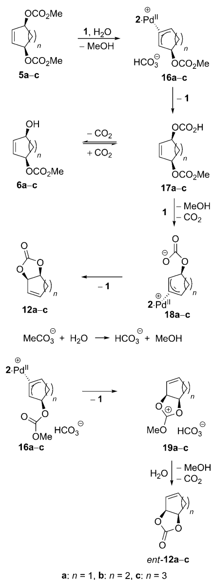
Scheme 8. Proposed mechanism for the Pd II -catalyzed formation of alcohol 6 and carbonates 12 and ent - 12 from bis-carbonate 5 .
