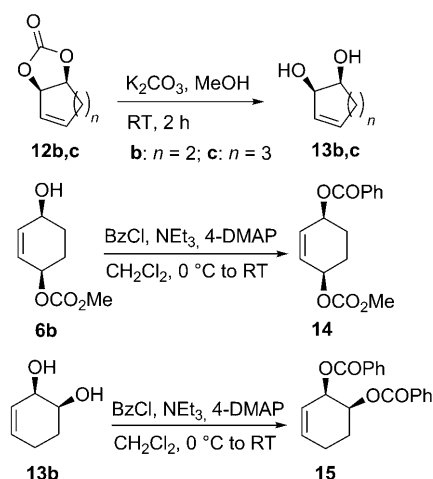
Scheme 7. Derivatization of the bicyclic carbonates 12b and 12c and alcohol 6b (4-DMAP = 4-dimethylaminopyridine, Bz = benzoyl).
