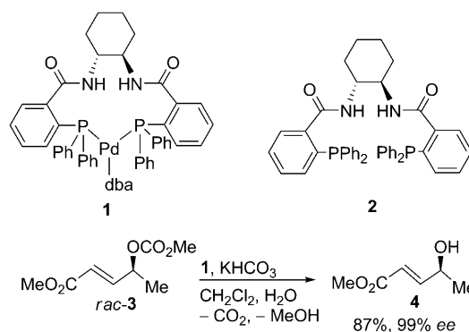
Scheme 1. Deracemization of the allylic carbonate rac - 3 with the Pd 0 complex 1 (dba = dibenzylideneacetone) and HCO 3 − in CH 2 Cl 2 and H 2 O.
