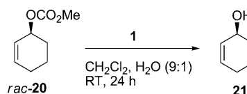
Scheme 10. Pd 0 -catalyzed deracemization of the monomethyl carbonate rac - 20 .
