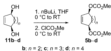
Scheme 4. Synthesis of the cyclic meso -biscarbonates 5b–d .
