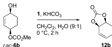
Scheme 9. Pd 0 -catalyzed synthesis of carbonate 12b from alcohol rac - 6b and CO 2 or HCO 3 − .
