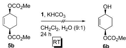
Scheme 5. Attempted Pd 0 -catalyzed desymmetrization of meso -biscarbonate 5b with 1 and HCO 3 − at room temperature.
