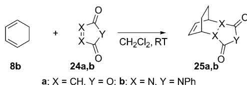
Scheme 14. Trapping of diene 8b as cycloadducts 25a and 25b .
