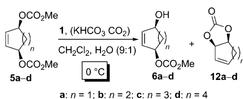
Scheme 6. Pd 0 -catalyzed desymmetrization of biscarbonate 5 with complex 1 and HCO 3 − at 0 °C.
