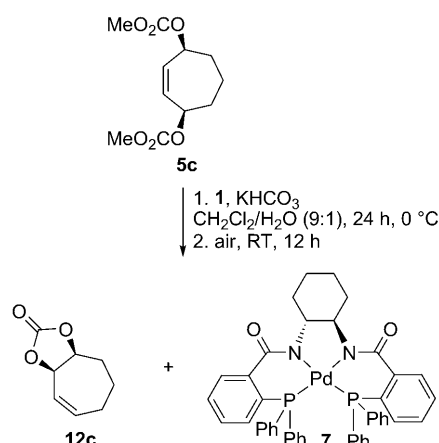
Scheme 15. Isolation of complex 7 in the desymmetrization of biscarbonate 5c with 1 through oxidative workup.
