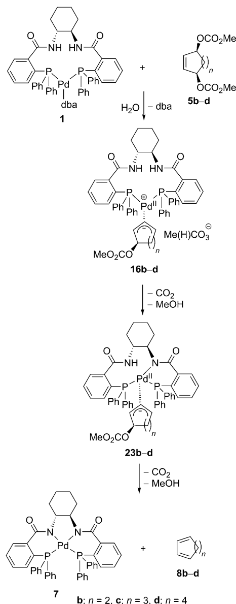
Scheme 13. Proposed mechanism for the redox reaction of the Pd 0 complex 1 with biscarbonate 5 .
