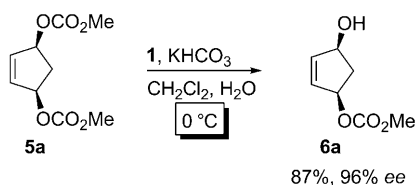
Scheme 2. \text{Pd}^0 -catalyzed desymmetrization of meso -biscarbonate 5a with complex 1 and \text{HCO}_3^- .
